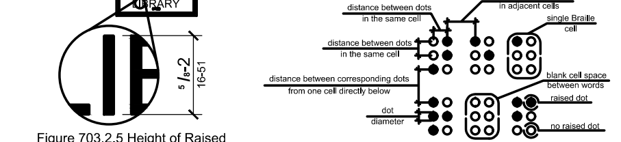
Figure 703.2.5 Height of Raised Characters
