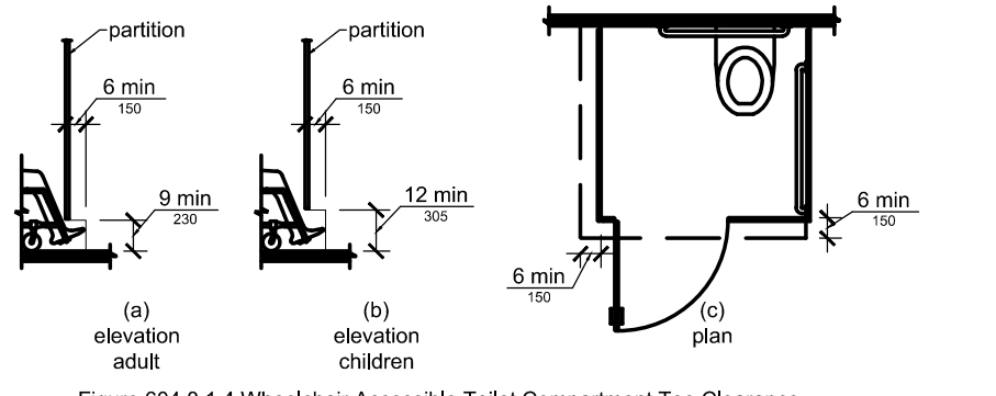
Figure 604.8.1.4 Wheelchair Accessible Toilet Compartment Toe Clearance
