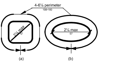
Figure 505.7.2 Handrail Non-Circular Cross Section
