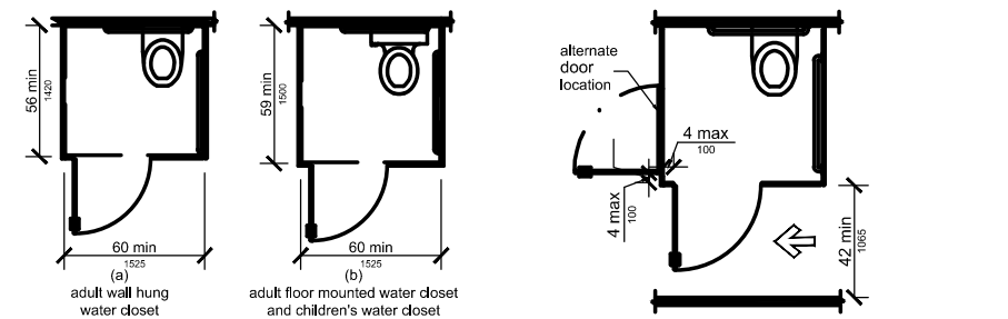
Figure 604.8.1.2 Size of Wheelchair Accessible Toilet Compartment
