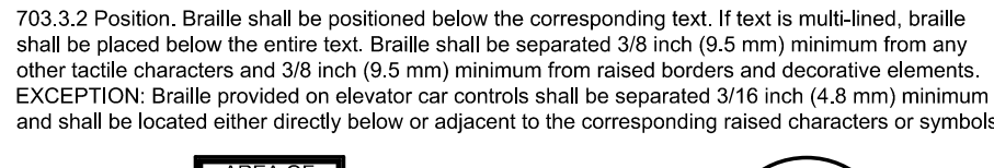
Figure 703.3.2 Position of Braille
