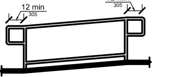
Figure 505.10.1 Top and Bottom Handrail Extension at Ramps
