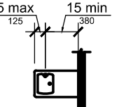
Figure 602.5 Drinking Fountain Spout Location
