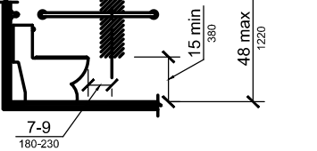
Figure 604.7 Dispenser Outlet Location
