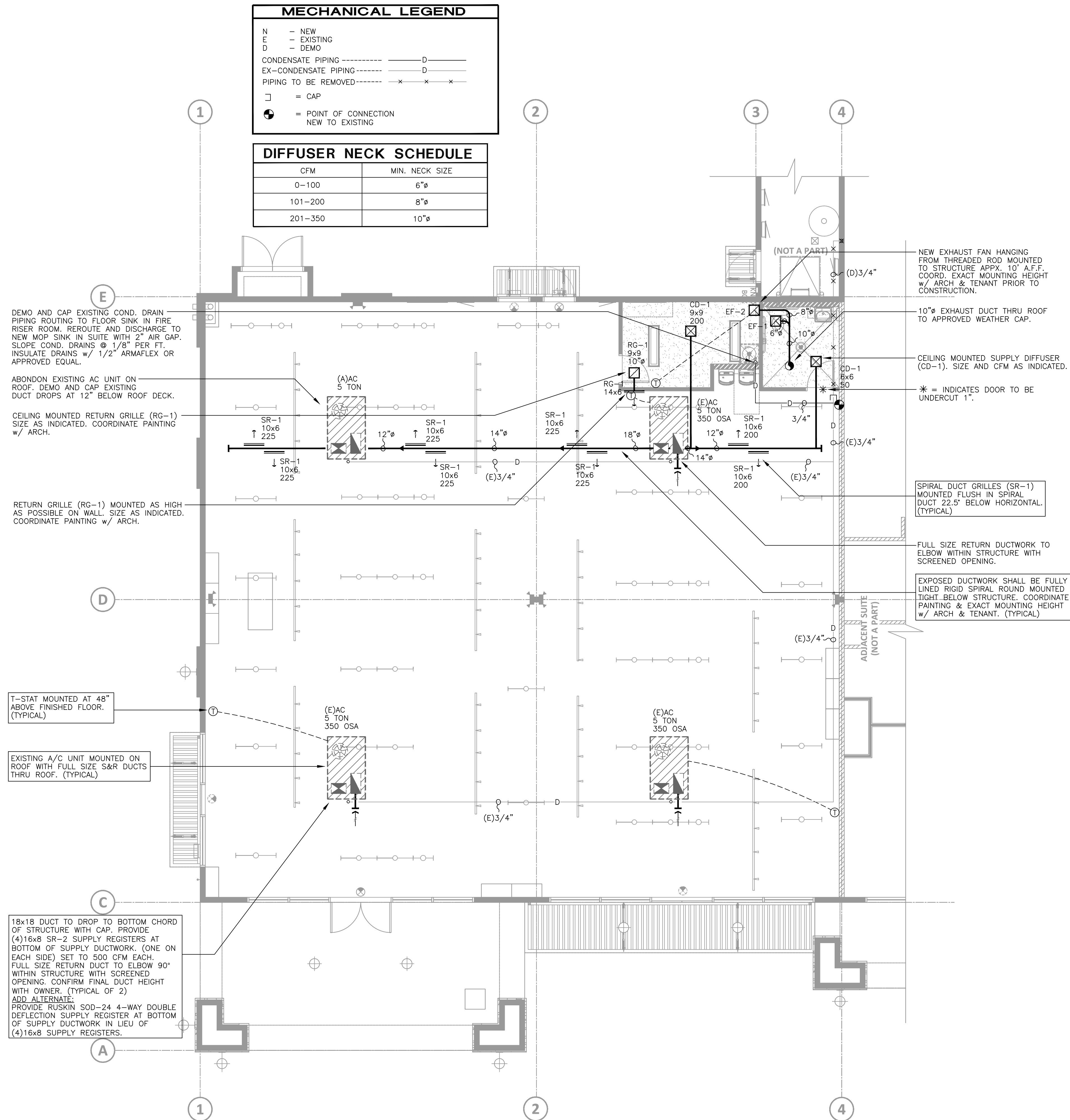
MECHANICAL FLOOR PLAN 3/16"=1'-0" NORTH
