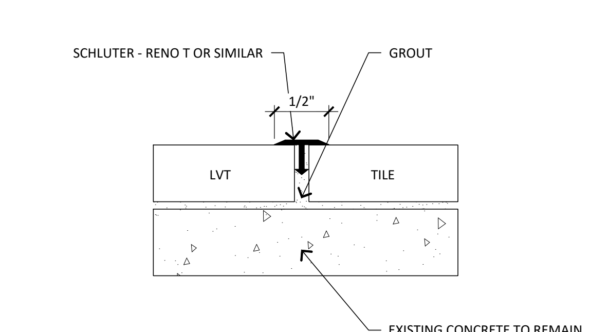
2 FLOOR TRANSITION; LVT TO TILE SCALE: 1'-0" = 1'-0"
