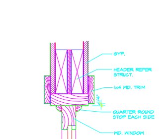
02 TYP. INTERIOR WIN. HEAD 3" x 1'-0"
