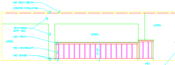
16 DINING 106 1/4"=1'-0"
