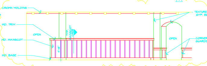
17 DINING 106 1/4"=1'-0"
