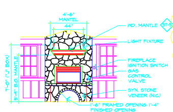
18 DINING 104 1/4"=1'-0"
