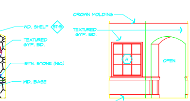
06 RECEPTION 102 1/4"=1'-0"
