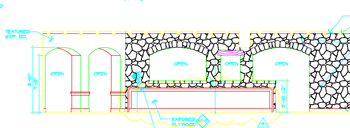
12 DINING 105/106 1/4"=1'-0"
