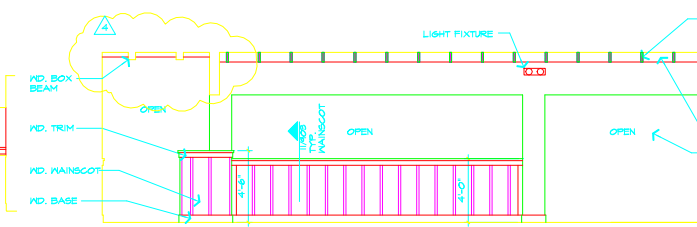
15 DINING 105 1/4"=1'-0"
