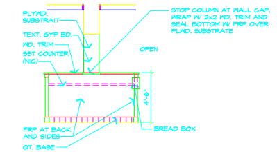
19 DRINK STATION 1/4"=1'-0"
