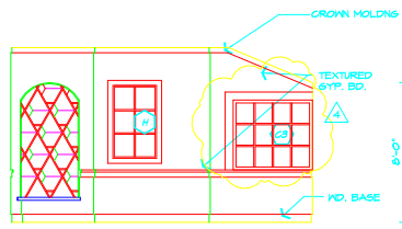
09 DINING 104 1/4"=1'-0"
