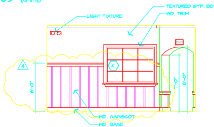
13 BAR DINING 107 1/4"=1'-0"
