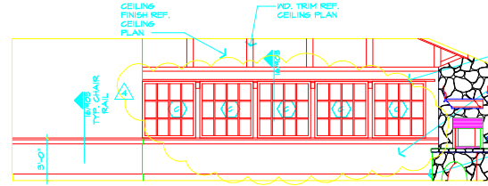
07 DINING 104 1/4"=1'-0"
