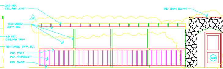
14 DINING 105 1/4"=1'-0"
