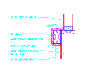
19 STUCCO TRIM AT SYN. BRICK 1 1/2"x1'-0"
