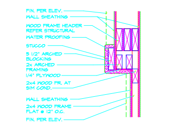
22 SILL AT SYN. STONE RECESS 1 1/2"x1'-0"
