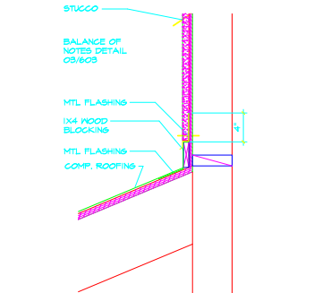
04 COMP. R.F.G. AT STUCCO WALL 1 1/2"x1'-0"
