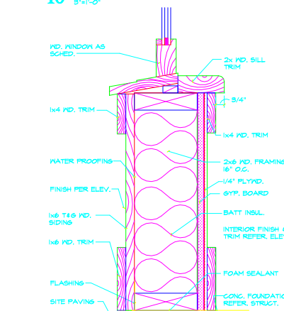
15 SILL WINDOW 'A-1' 3'1"-0"
