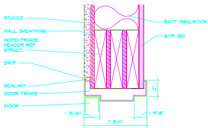
05 HEAD DOOR 114, 118, 119, 123 3'1"-0"
