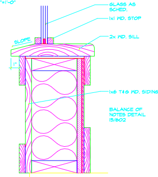
13 SILL WINDOW 'F' 3'1"-0"
