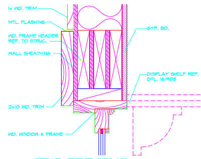
02 HEAD WINDOW 'C' 3'1"-0"
