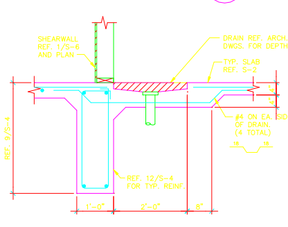
18 RECESS AT MOP SINK SCALE: 3/4"=1'-0"
