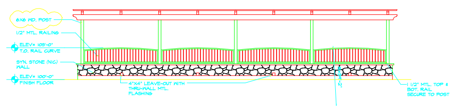
03 PATIO ELEVATION 1/2"=1'-0"
