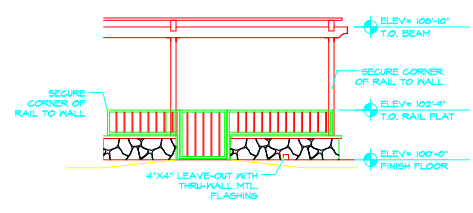
04 PATIO ELEVATION 1/4"=1'-0"
