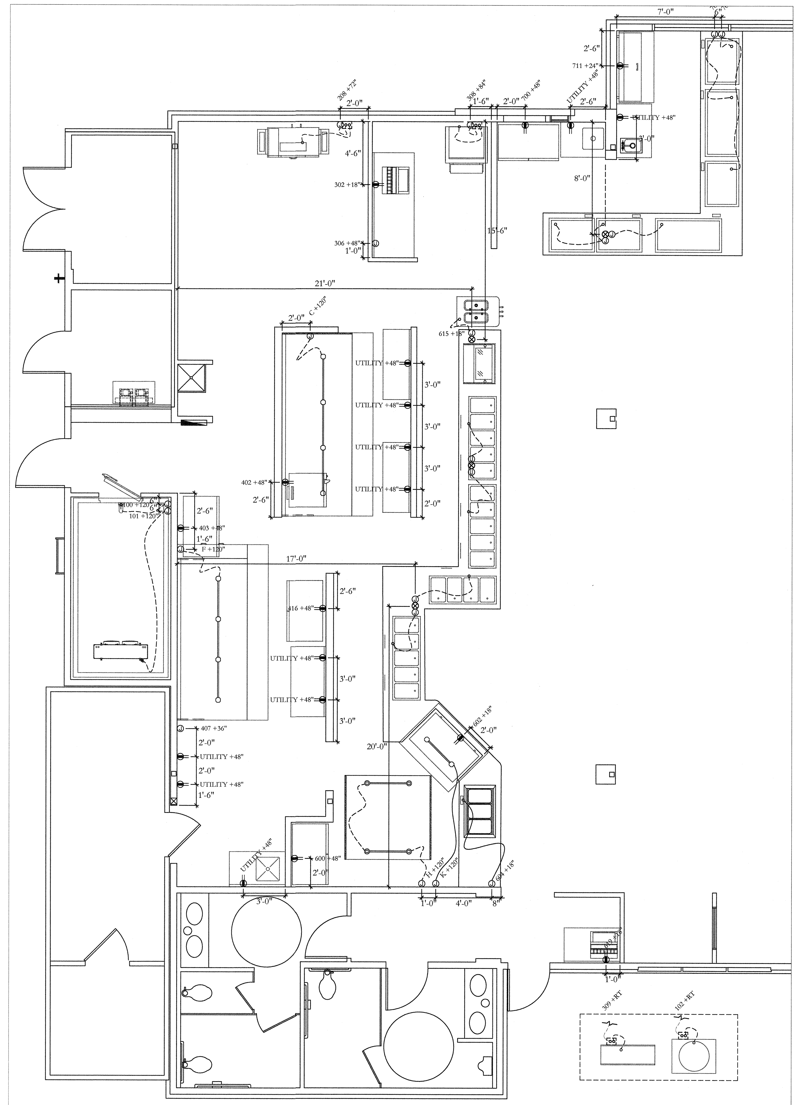
ELECTRICAL ROUGH IN PLAN SCALE: 1/4"=1'-0"
